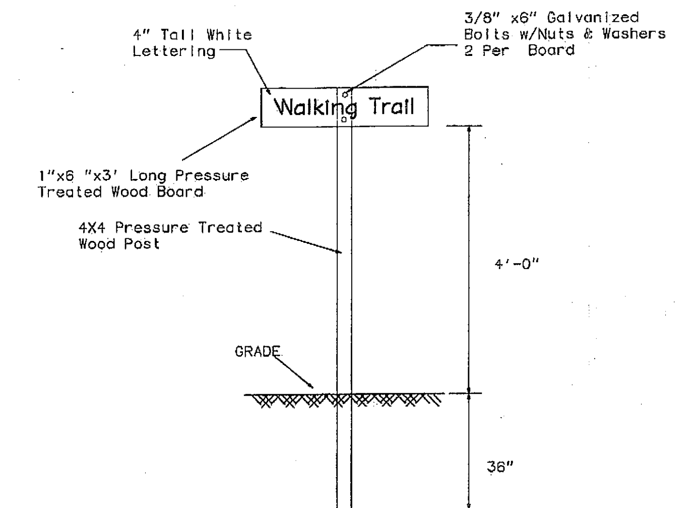
WALKING TRAIL SIGN DETAIL
