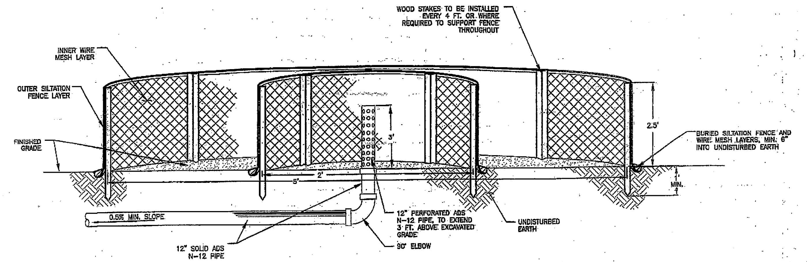
SILT FENCE BAFFLE RING AND PERFORATED PIPE TEMPORARY SEDIMENT BASIN
